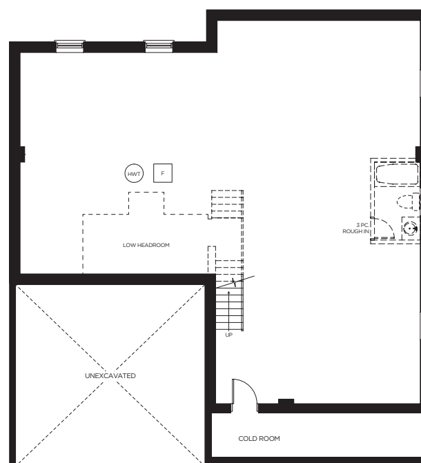
BASEMENT PLAN
