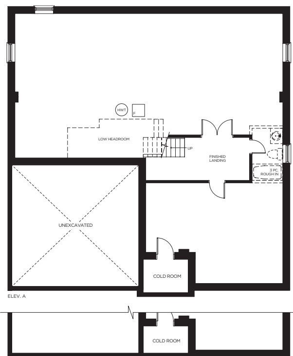
BASEMENT PLAN
