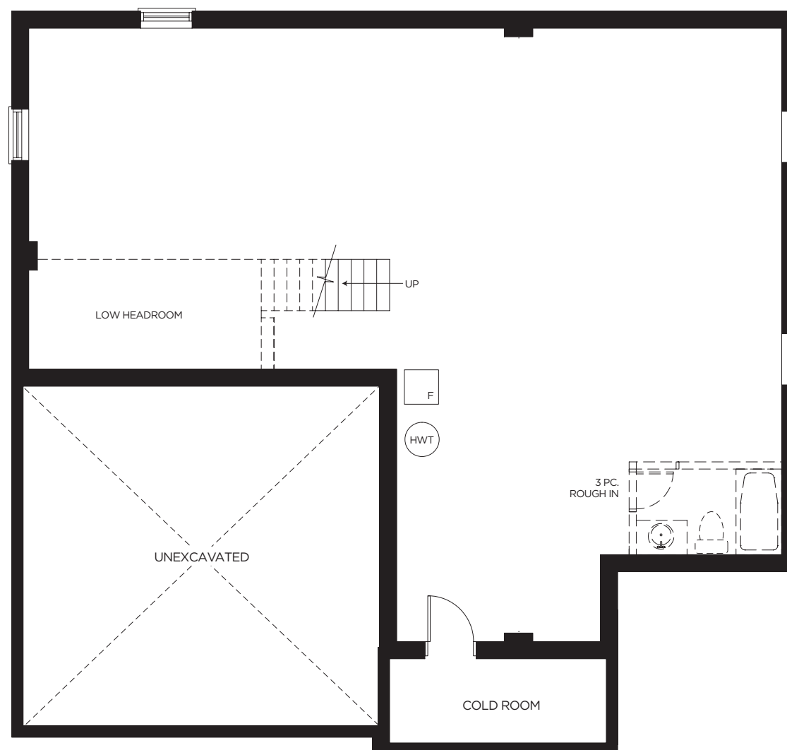
BASEMENT PLAN
