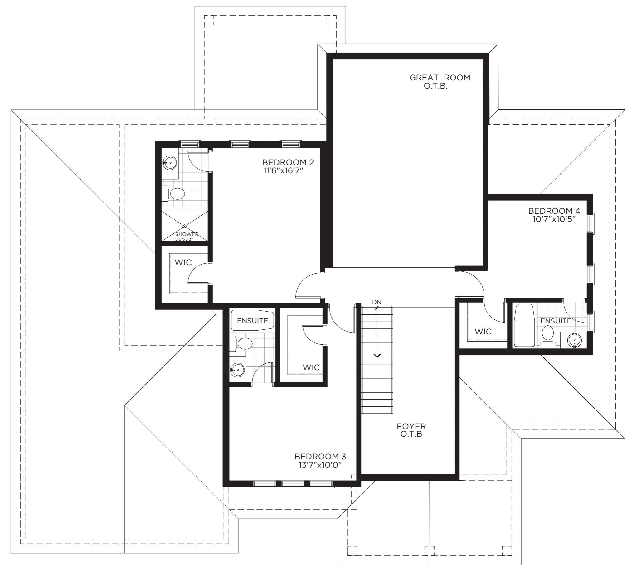
SECOND FLOOR PLAN ELEV. A
